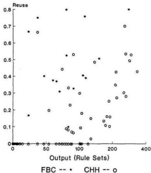
Fig. 7. Reuse and programmer output.
