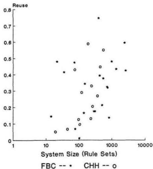
Fig. 6. Reuse and system size.
