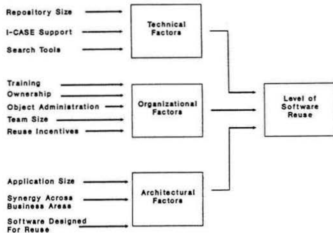
Fig. 8. A revised model of reuse.
