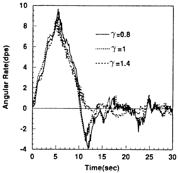
Figure 7 Experimental results for the slow maneuver of Flexible Spacecraft Simulator
