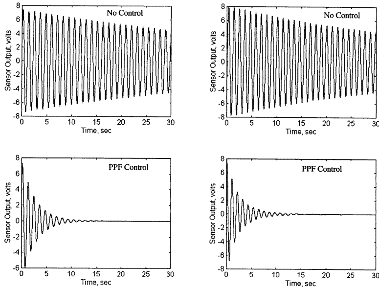
Figure 11. Simulation (left) and experimental results (right) of implementing a PPF controller on a second-mode excitation.
