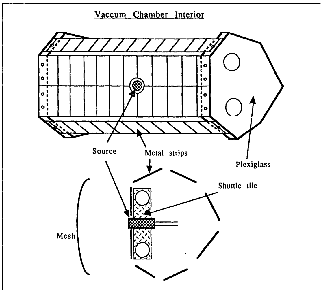
Figure 16. Vacuum chamber interior
