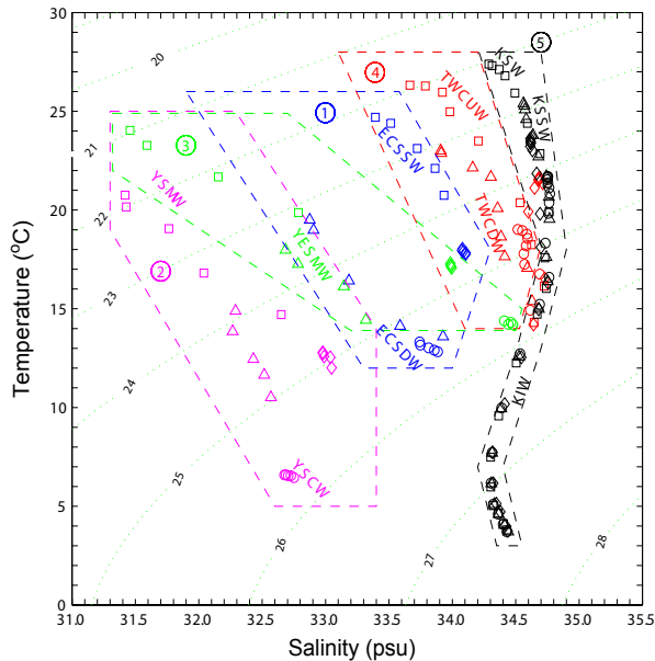
Fig. 14. Water mass classification on the climatological T - S diagram.
