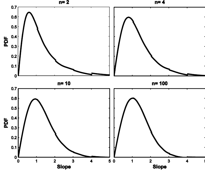
Fig. 2. The s-PDFs for various surface characteristics: (a) n = 2 , (b) n = 4 , (c) n = 10 , and (d) n = 100 .
