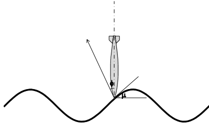
Fig. 3. Ocean surface inclination angle ( \mu ) and bomb impact angle ( \phi ) relative to the normal direction of the surface.
