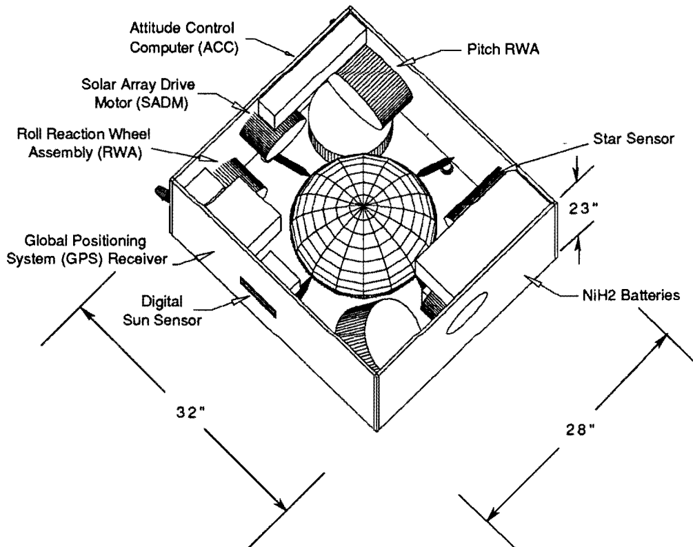
Figure 1. MPS Configuration.
