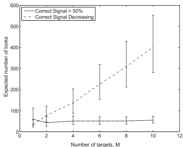
Fig. 9. Expected number of looks until the sequential eliminating procedure terminates as M increases for two different categories of the sensor matrices S_i , A = 10 , \alpha = 0.05 and M ranges from 1 to 10.
