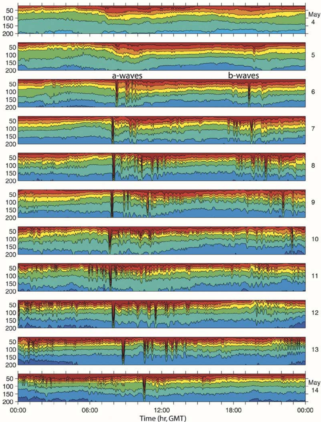
Fig. 4. Stack plot of temperature at mooring S7 on the 350 m isobath. The bottom 150 m are not shown to allow a clearer presentation of the internal wave structure. All available temperature sensors (Fig. 2, Table I) were used to construct the plot. Each panel is one day (May 4–14, 2001) from 0000 to 2400 h.
