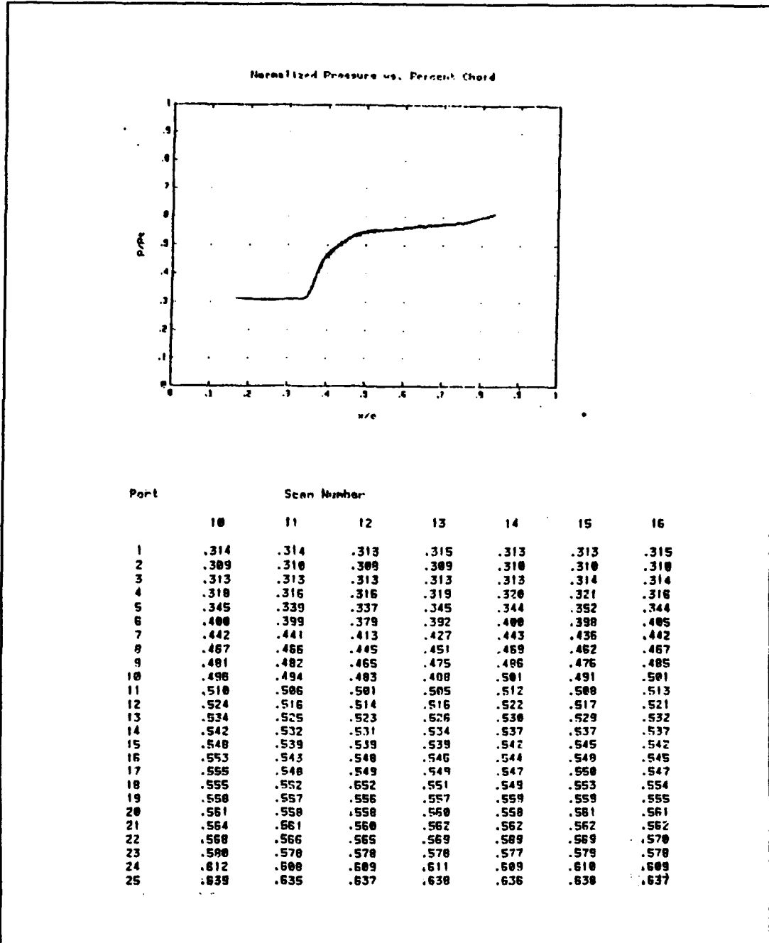
Figure D3. (cont) Run 7, 6-25-93, ZOC #1 (Lower Blade Pressure Distribution)
