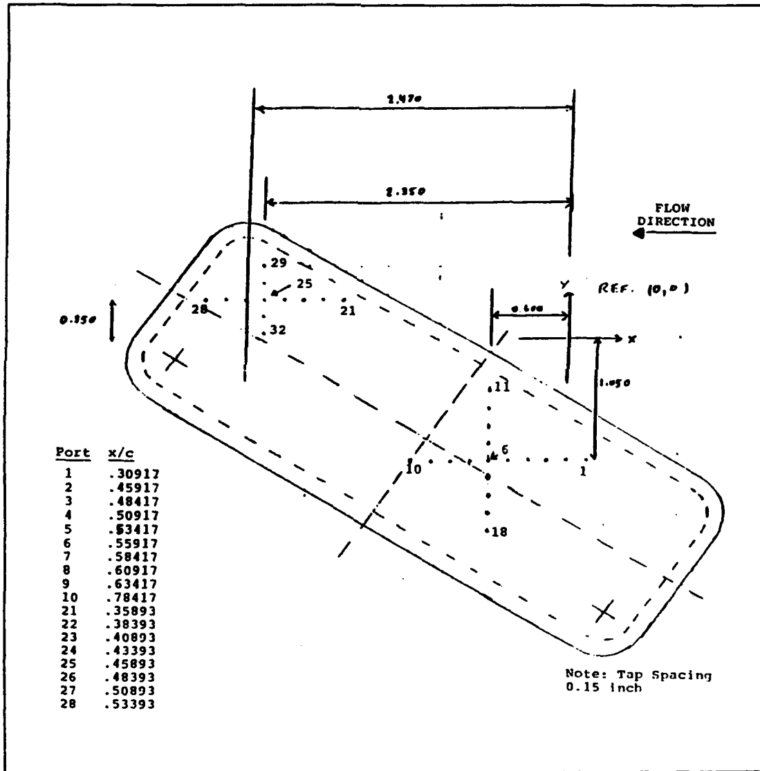
Figure A1. Left-Hand Window Blank Pressure Taps
