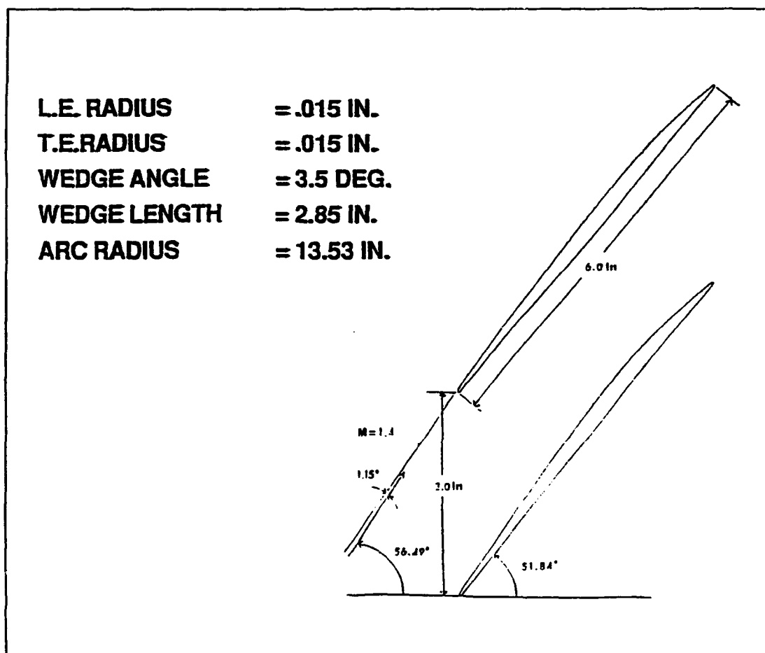
Figure 4. Transonic Cascade Blade Geometry
