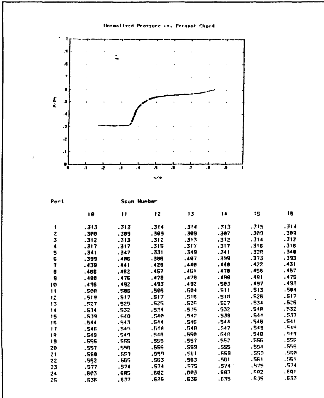
Figure D1. (cont) Run 5, 6-25-93, ZOC #1 (Lower Blade Pressure Distribution)
