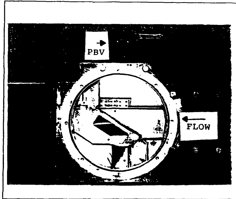
Figure 5. Test Section
