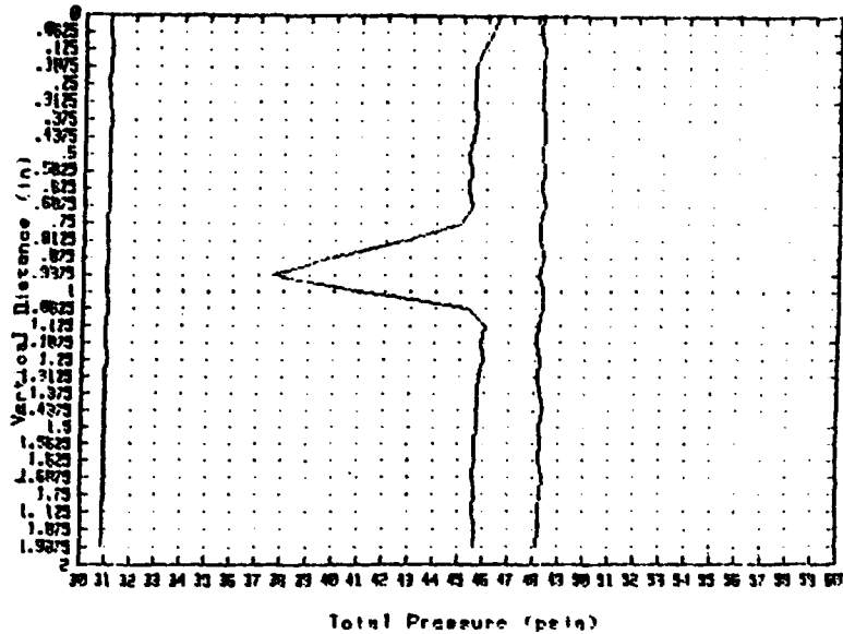
Vertical Distance Traversed vs. Pt
