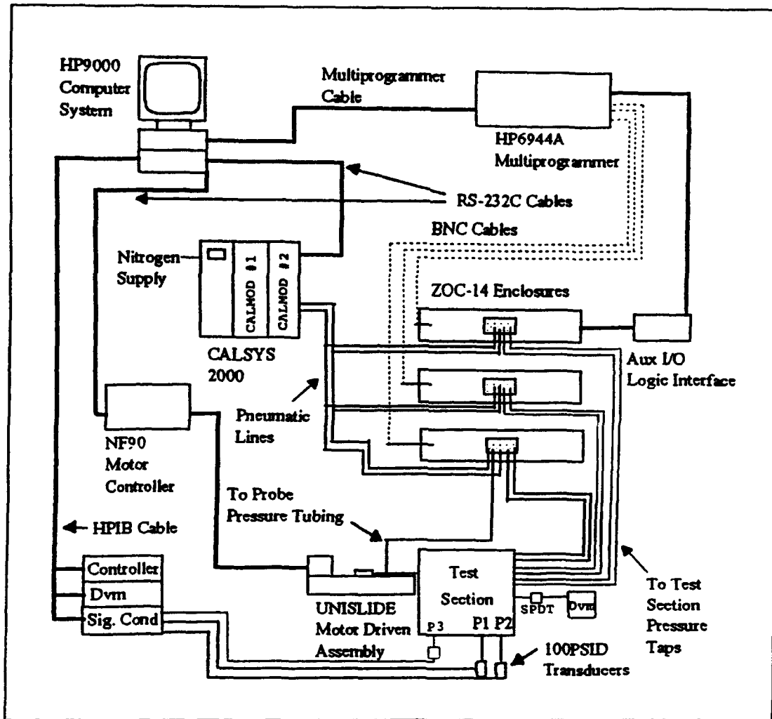
Figure 7. Data Acquisition Schematic
