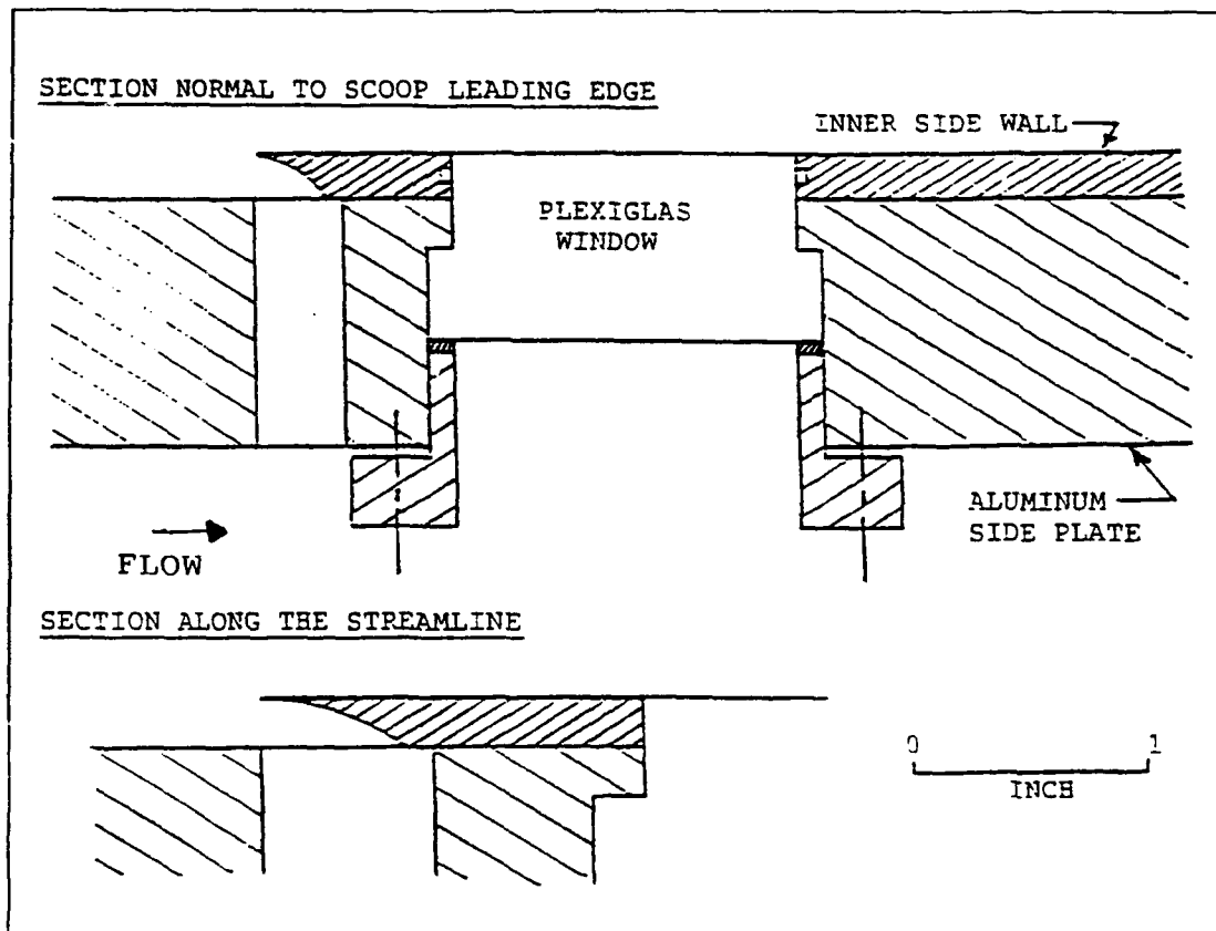
Figure 6. Boundary Layer Diversion
