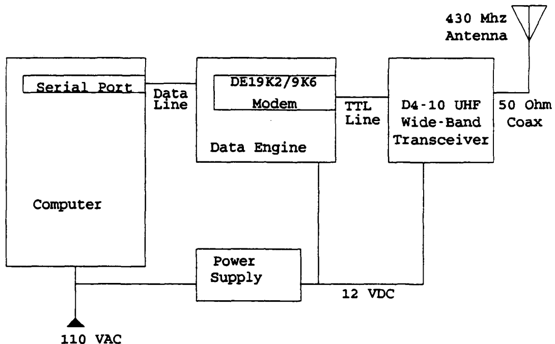
Figure 15 Ground Station Packet Radio Data Link Block Diagram .
