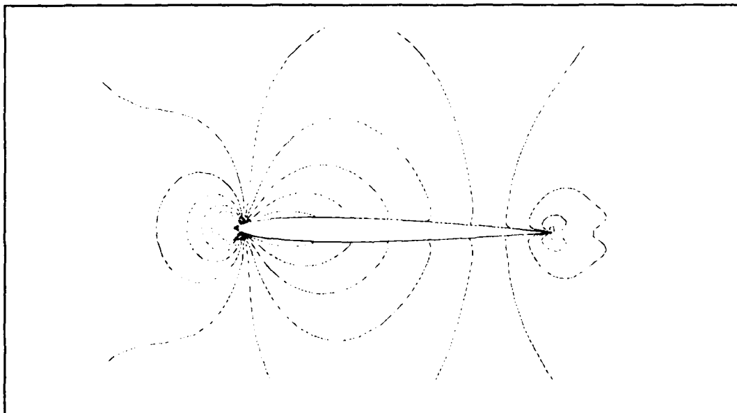
Figure 6.1 : Mach Contours around NACA 0008 Baseline Airfoil
