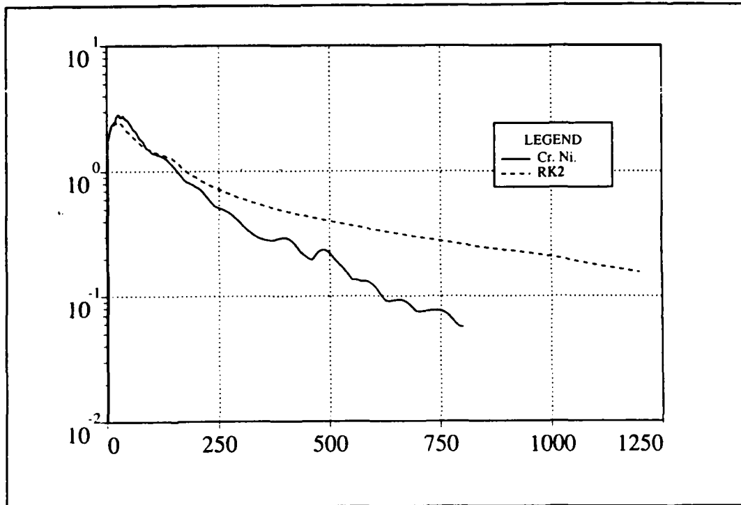
Figure 3.12 : Convergence History for Crank-Nicholson and Runge-Kutta Schemes
