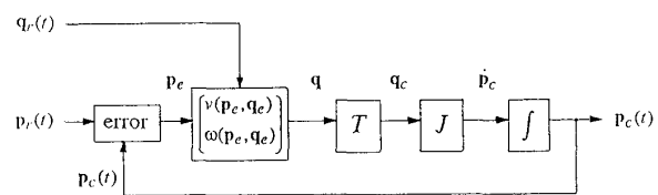
Fig. 3 Architecture of Tracking Controller
