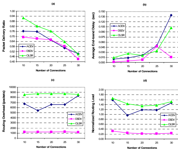
Figure 8. Results of varying number of data connections on (a) PDR (b) average end-to-end delay (c) ROH and (d) NRL
