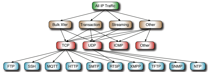
Fig. 5: Application-profile lattice
