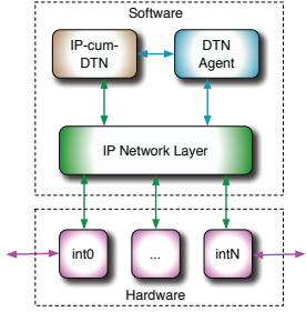
Fig. 3: IP-cum-DTN gateway architectural components
