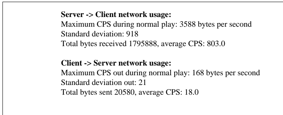
Figure 10. Server vs. client communication in Netrek.
