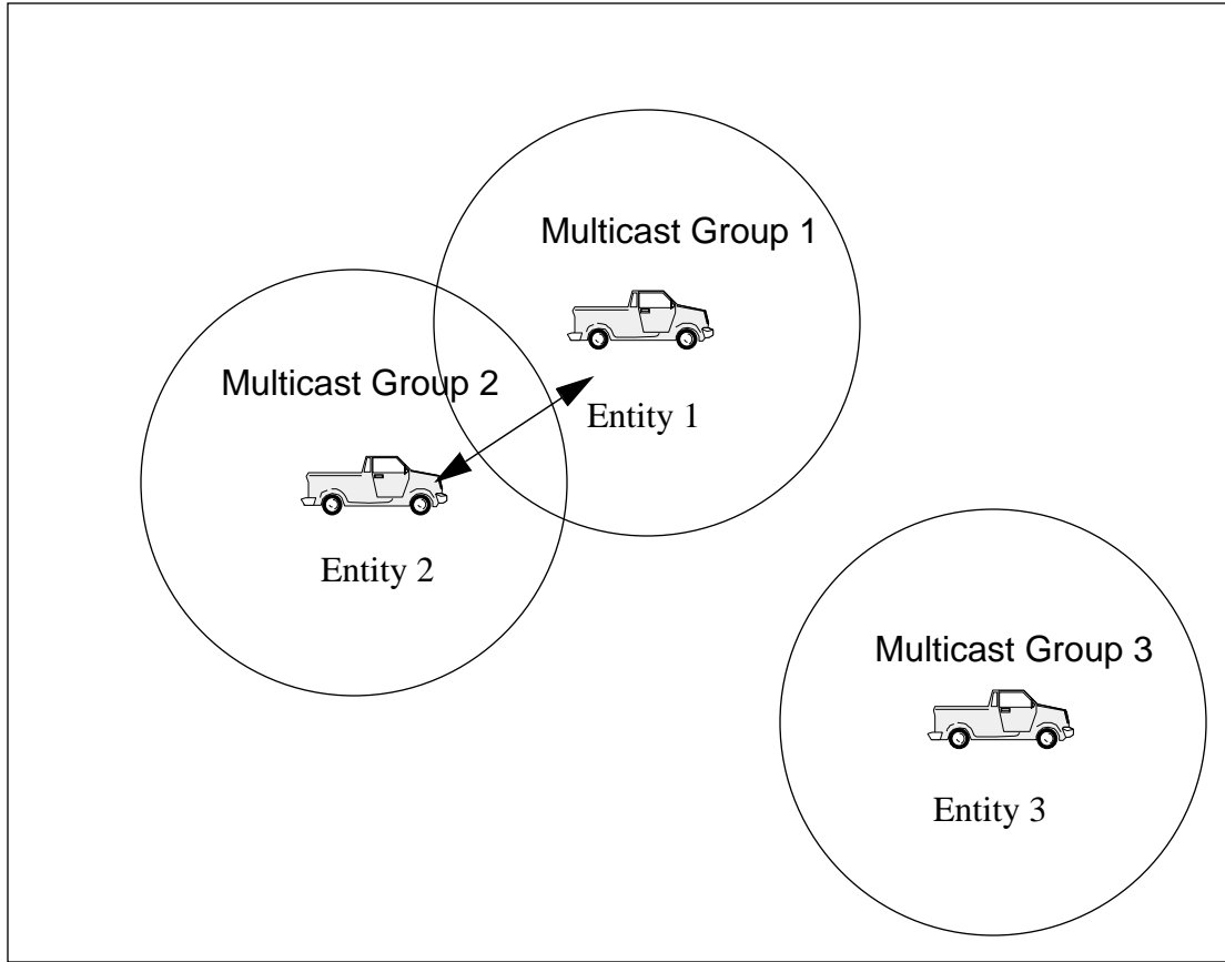
Figure 6. Object-based filtering.
