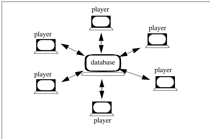
Figure 9. Centralized model.
