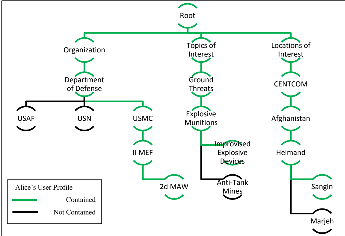
Figure 9. Example characteristic tree.
