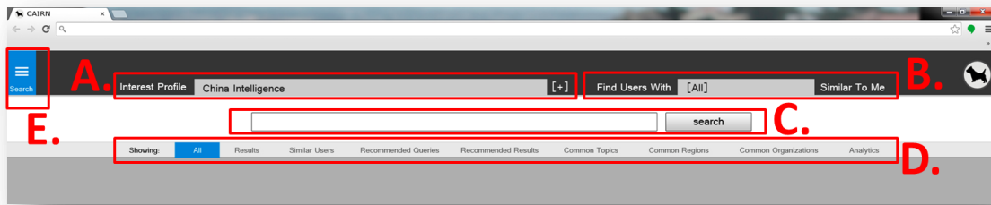
Figure 17. Search Configuration
