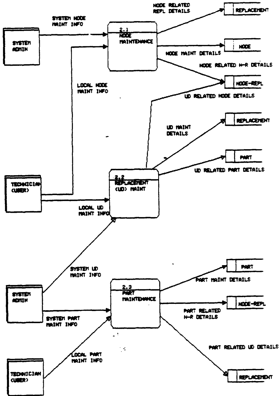
Figure B-9 - DFD: Data Store Maintenance Subsystem [2.0]
