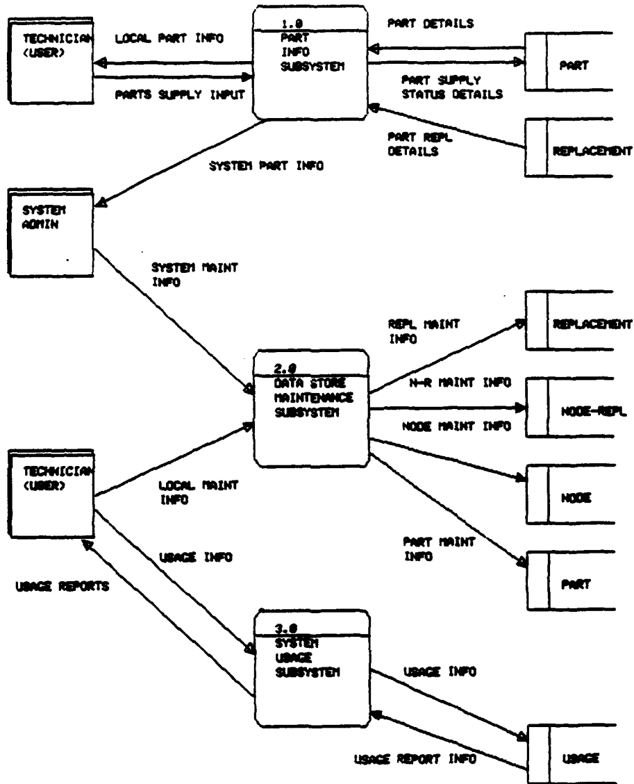
Figure B-6 - MK92 FCS MAES DB System Diagram
