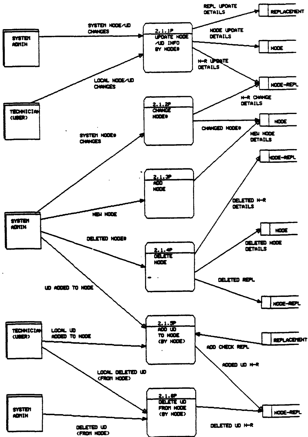
Figure B-10 - DFD: Node Maintenance [2.1]
