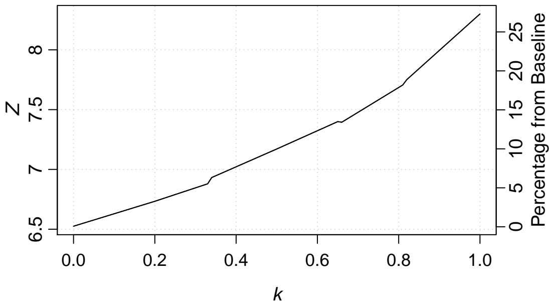
Figure 4.3: Objective value of the robust formulation for optimistic priorities as a function of k .
