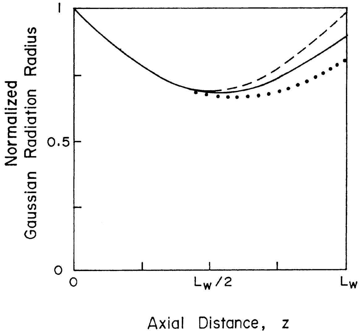
Fig. 7. Normalized 1/e Gaussian radiation field amplitude radius as a function of distance z in the wiggler with \lambda = 1.25 \mu\text{m} and edge emittance \epsilon_N = 10 \text{ mm mrad} for three different currents: (- - -) I = 0.5 \text{ A} , (—) I = 2 \text{ A} and (.....) I = 4 \text{ A} .
