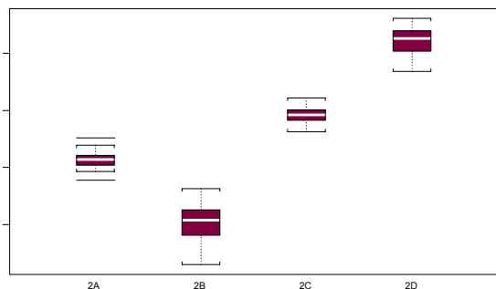
Figure 5: Boxplot of FCS COA's
