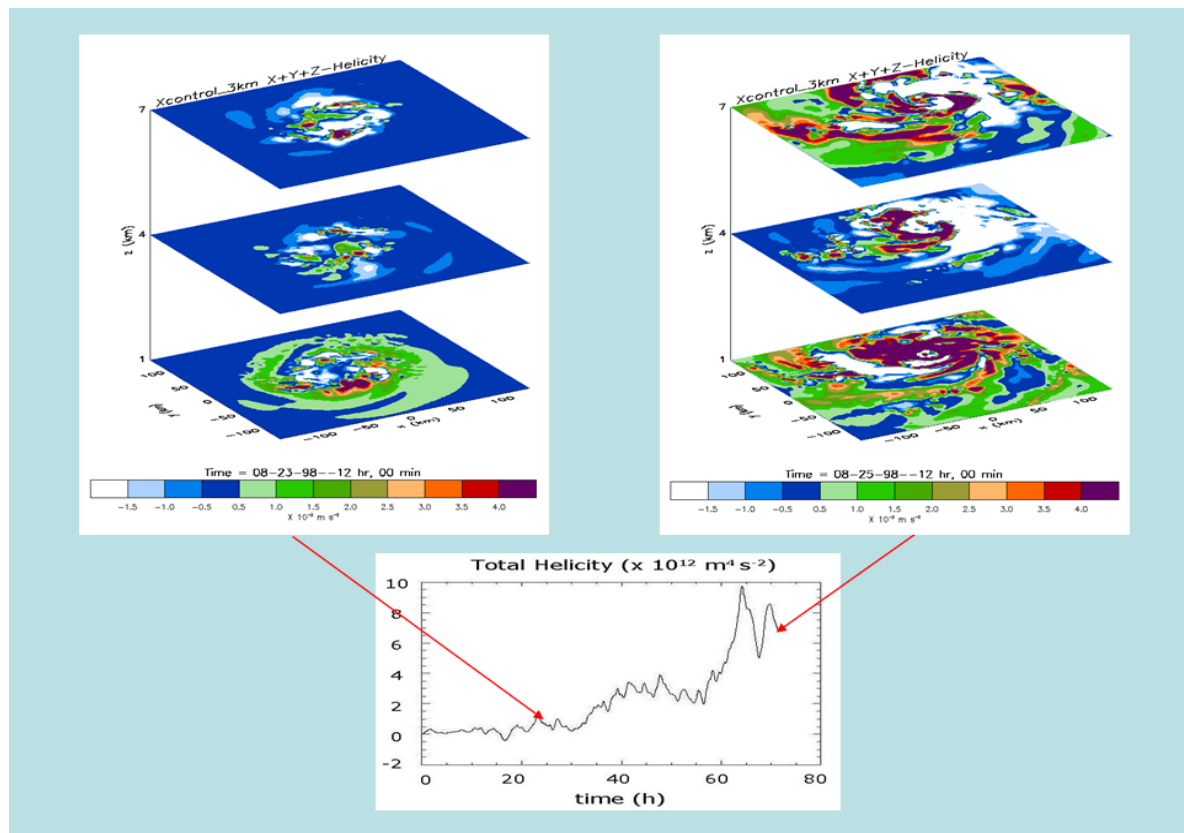
Figure 2. Helicity density ( \times 10^{-4} \text{ m s}^{-2} ) in three horizontal cross-sections of 276 \times 276 \text{ km}^2 at z = 1, 4, 7 km is shown for tropical depression (left) and mature hurricane (right), and mean total helicity ( \times 10^{12} \text{ m}^4 \text{ s}^{-2} ) integrated over the computational domain 276 \times 276 \times 20 \text{ km}^3 during 72 hours of hurricane vortex evolution is given in the lower panel.
