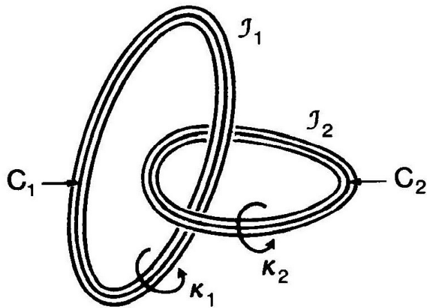
Figure 1. Prototype configuration of linked vortex lines that gives nonzero helicity. Borrowed from (Moffatt & Tsinober, 1992).
