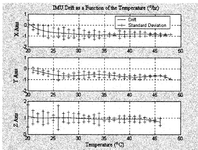
Fig. 3. Gyro drift approximation. The red bars represent the standard deviation as observed in different trials.
