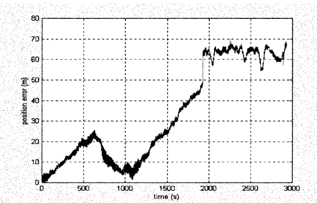
Fig. 12. Position error in full dead-reckoning mode.
