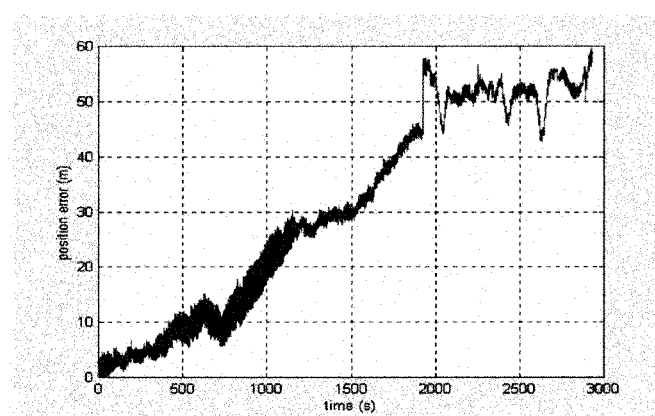
Fig. 13. Position error without compass.
