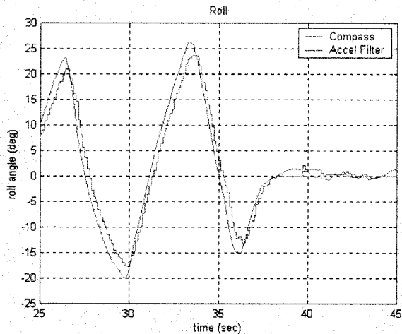
Fig. 5. Roll estimation in a moving environment ( ^{\circ} ).
