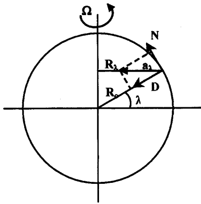
Fig. 2. Earth rotation.
