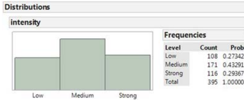
Figure 4. Intensity distribution of the study data set.
