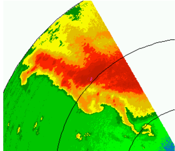
Figure 5. Radar reflectivity of the Greensburg, KS supercell on 4 May 2007, as seen by UMass X-Pol at 2049 CDT at 4.2^\circ elevation angle. Range markings are spaced apart every 10 \text{ km} . The nearest range marker is at 10 \text{ km} . The radar was located \sim 4 \text{ km} east of Protection, KS.
