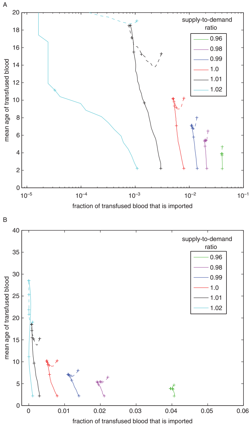
Fig. 3. Two tradeoff curves (a solid curve for the Type I patients that have a discretionary threshold and a dashed curve for the Type II patients that have a threshold of 42 days) for various values of the supply-to-demand ratio, with the import rate on a (A) logarithmic and (B) linear scale. The four tick marks on each curve correspond to threshold values (for the Type I patients with a discretionary threshold) of 2, 14, 28, and 42 days. Because 500,000 transfusions were simulated to generate each point on these curves, we are not able to accurately estimate import rates of less than 10 -5 .
