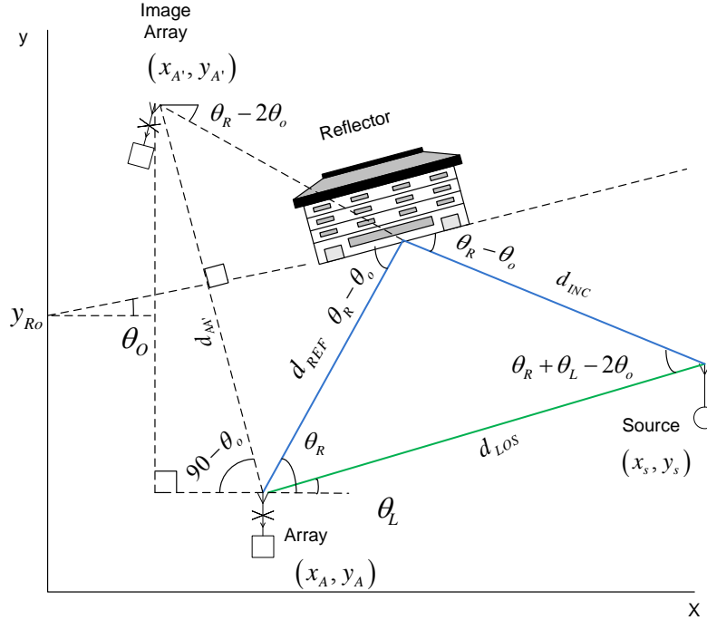
Figure 23. Single-array, single-source, single-reflector scenario used to illustrate the expected TDOA relationship between the LOS and the NLOS signal.
