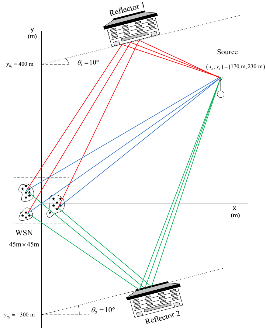
Figure 36. Scenario 2: Single source located at (170 \text{ m}, 230 \text{ m}) . Two reflectors, both with orientation \theta = 10^\circ and reference point at y_{R_1} = 400 \text{ m} and y_{R_2} = -300 \text{ m} respectively. A variable number of arrays were randomly distributed in a 2025 \text{ m}^2 square area.
