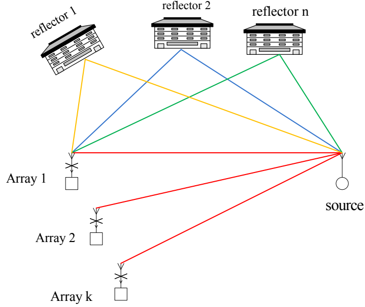
Figure 26. Single-source localization using multiple arrays in the presence of multiple reflectors.
