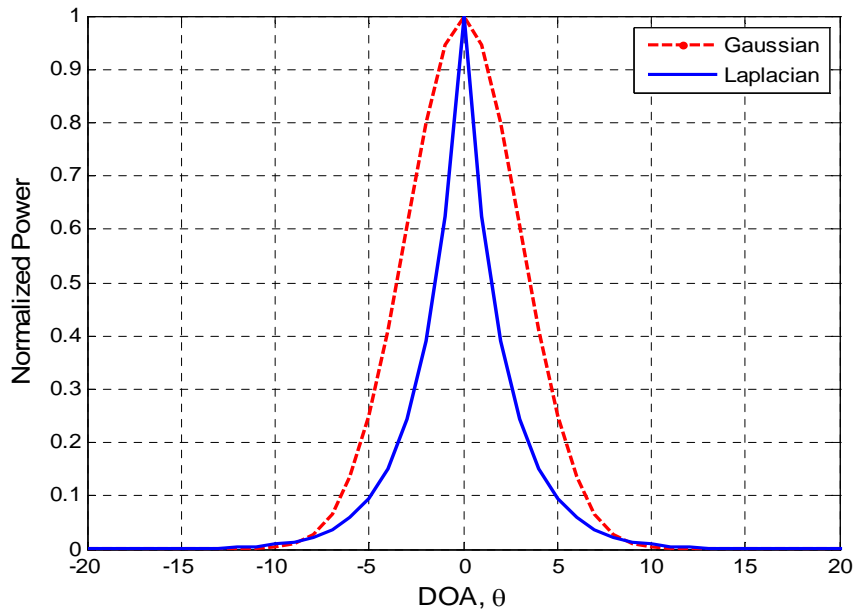
Figure 8. Gaussian versus Laplacian scattering functions.
