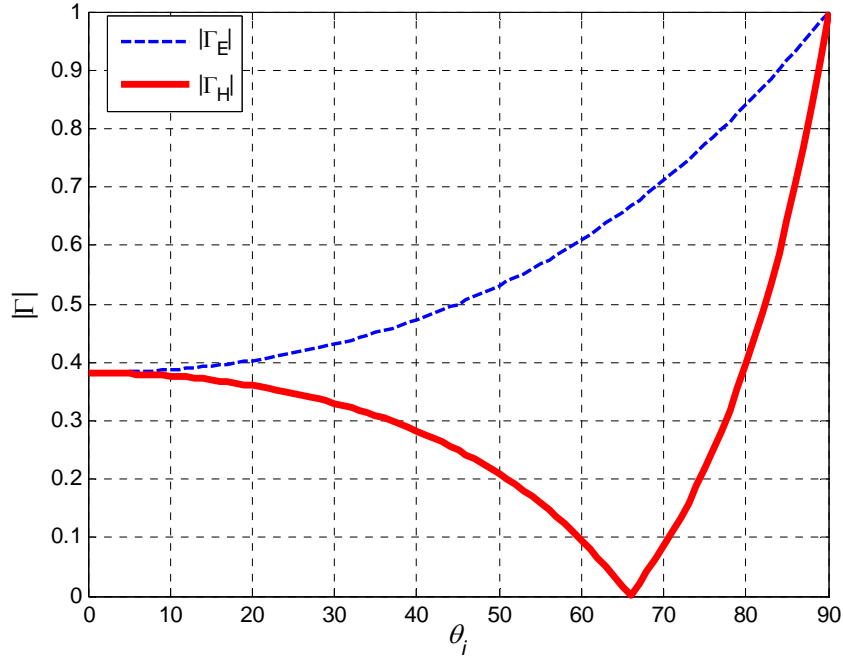
Figure 5. |\Gamma| as a function of the incident angle for \epsilon_r = 5 .
