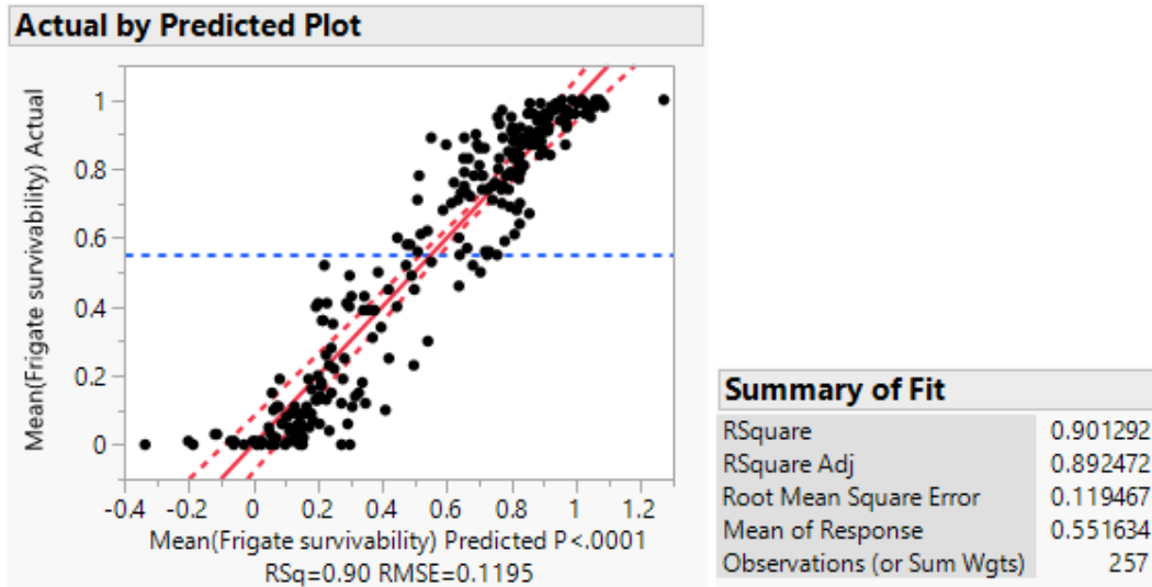
Figure 24. Actual by Predicted Plot and the Summary of Fit for the Second Order Model.
