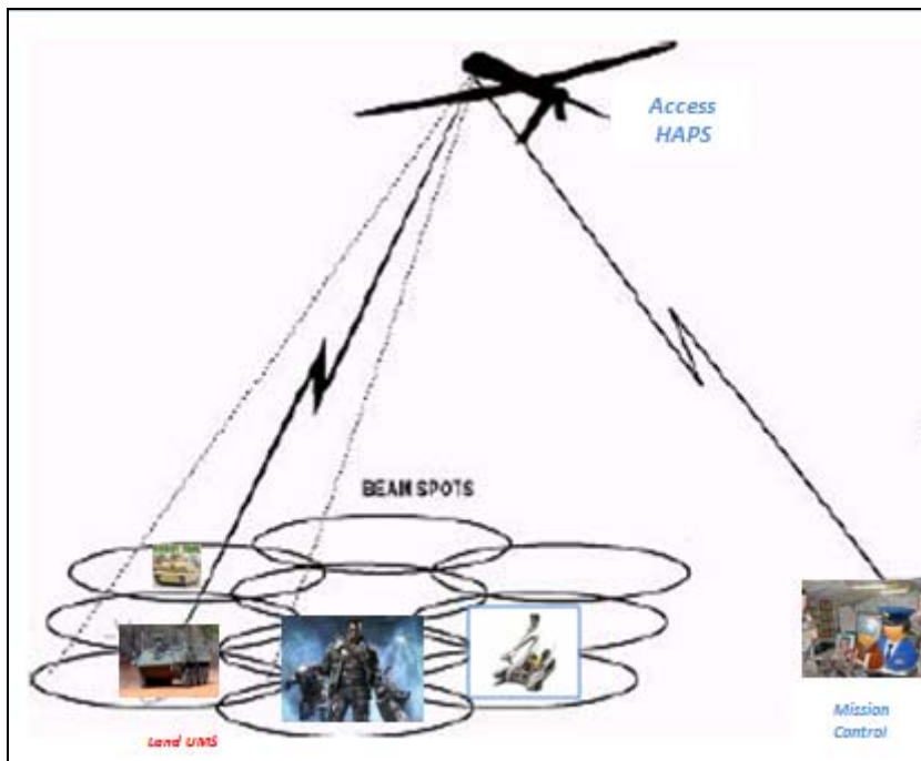
Figure 66. Access HAPS 201
