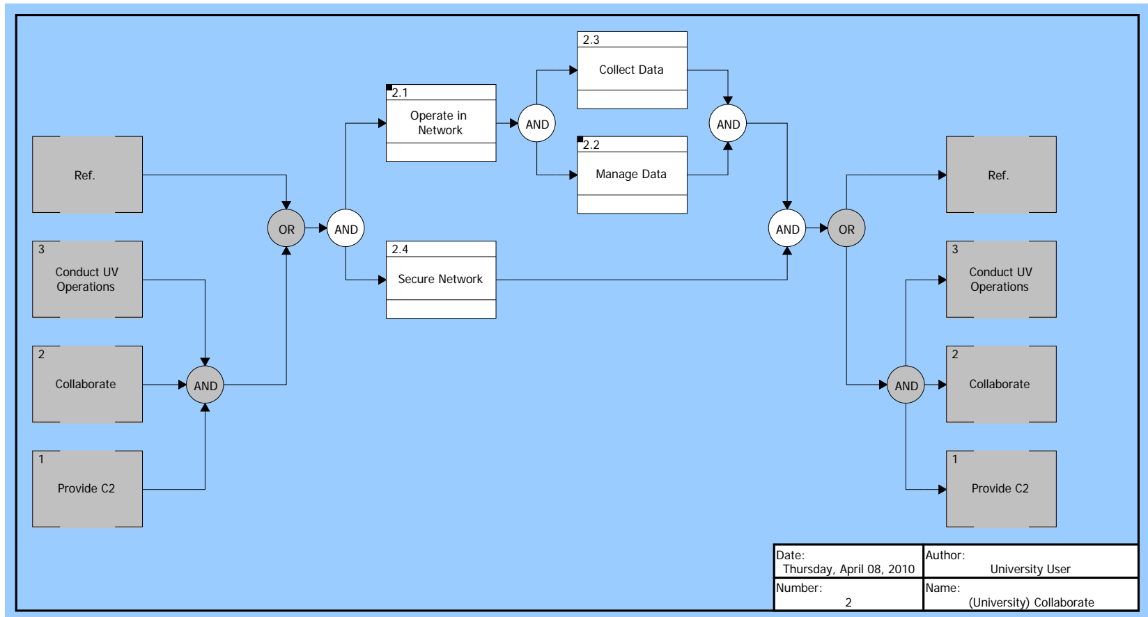
Figure 48. Collaborate FFBD
