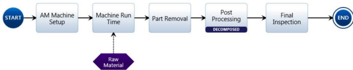
Figure 28. AM Process Flow Diagram
