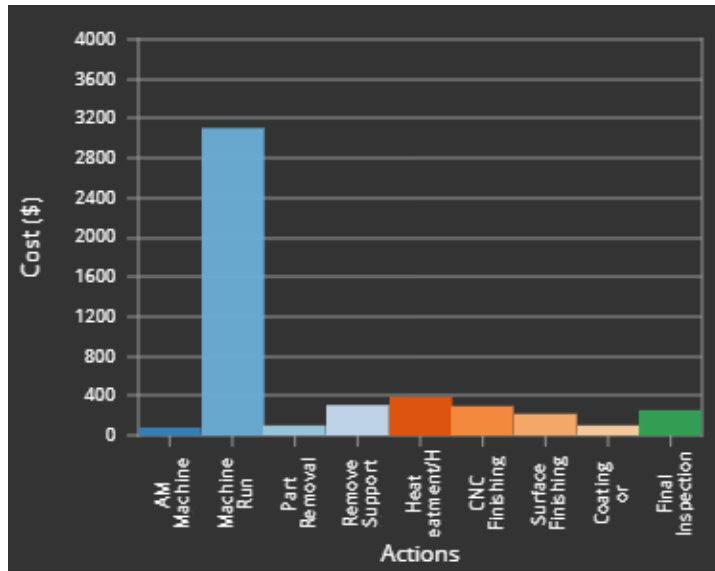
Figure 33. Innoslate DES Cost Breakdown for Half Print Speed
