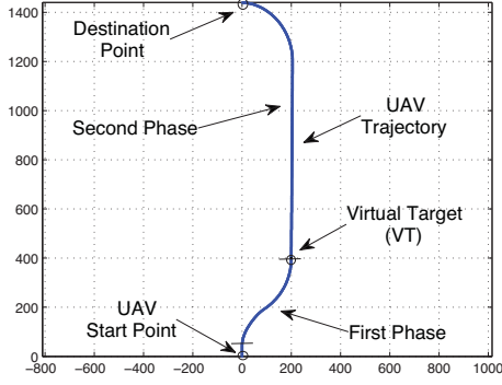
Fig. 5. UAV trajectory in mission for stationary destination
