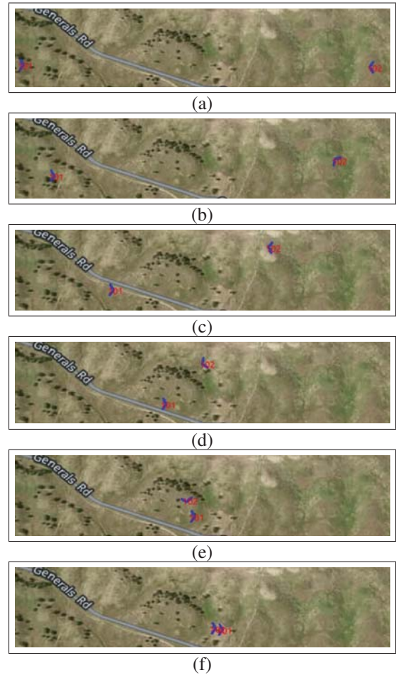
Fig. 7. Snapshots of an illustrative run of the software-in-the-loop (SITL) simulation environment of the UAV-UAV engagement benchmark problem. (a) The target UAV starts from the west and transits east; (b) the pursuer UAV maneuvers towards a virtual point, to (c) align on a parallel course; (d) the pursuer UAV turns into the target UAV, (e) achieving an intercept heading, and (f) resulting in a successful tail-chase engagement.
