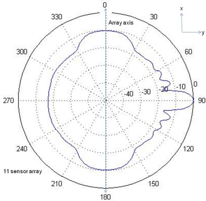
Figure 28 Cardynull Response to Signal and Noise (SNR = 0 dB)
