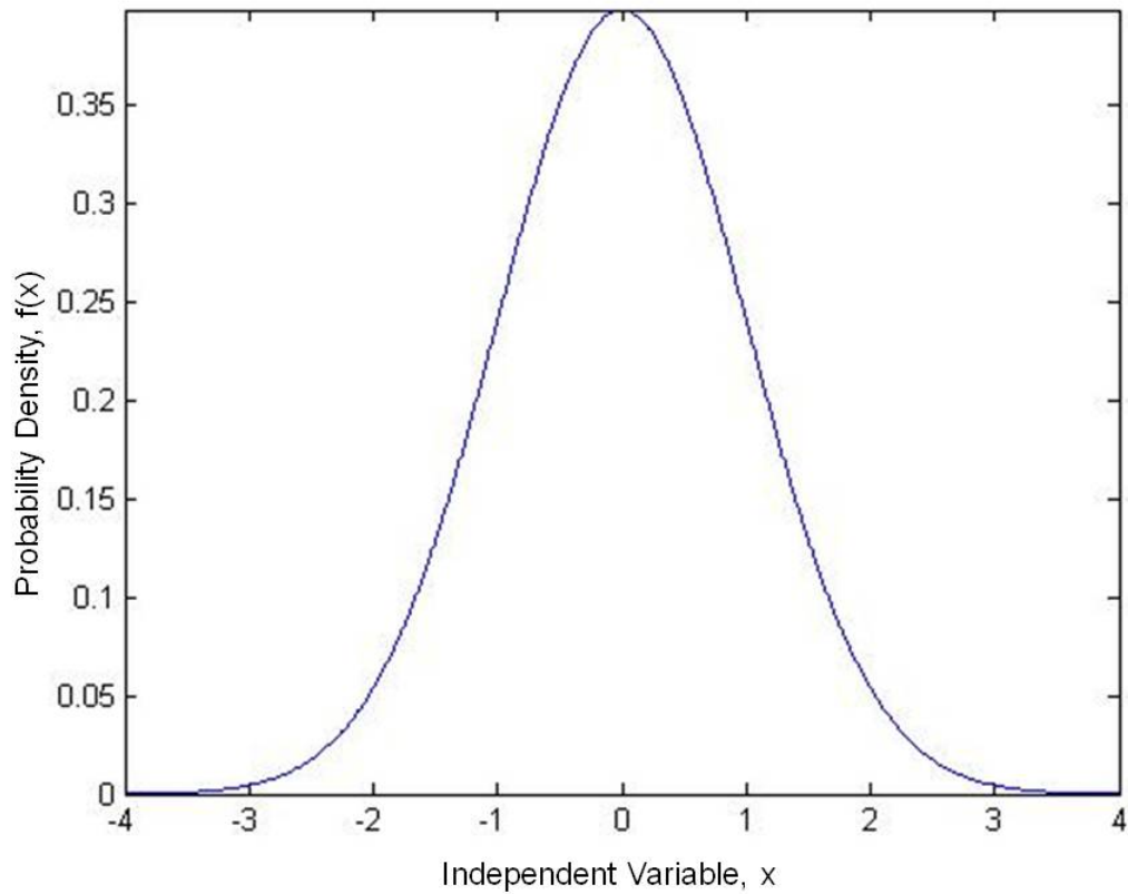
Figure 16 Probability Density Function for \mu = 0, \sigma^2 = 1
