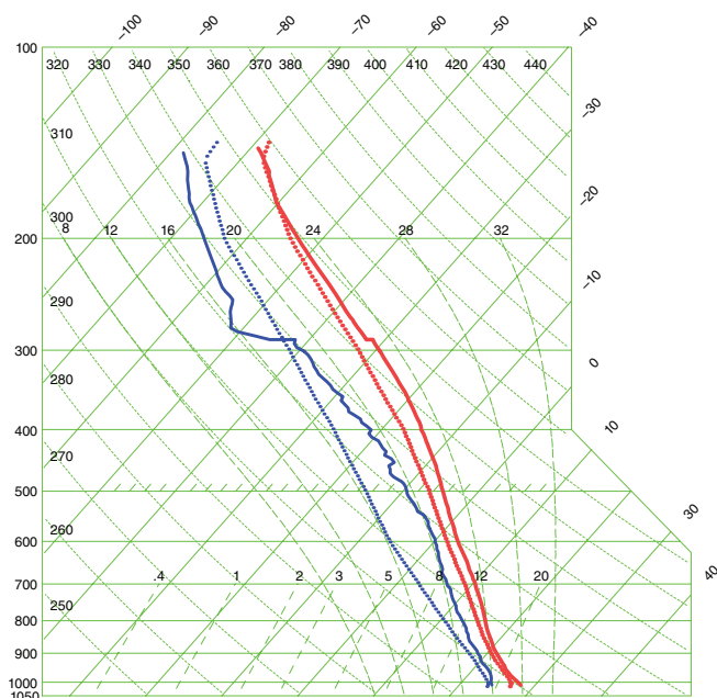
Figure 1. Skew T – \log p diagram showing the temperature (right solid curve) and dew-point temperature (left solid curve) of the Karl pouch sounding used in this study. Also shown is the Dunion moist tropical sounding with temperature (right dotted curve) and dew-point temperature (left dotted curve), which is used for one of the sensitivity experiments.
