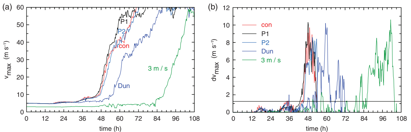
Figure 9. Time series from five experiments of (a) maximum azimuthally averaged tangential wind speed ( V_{\max} ) and (b) the 2 h tendency, dV_{\max}(t) = V_{\max}(t+2\text{ h}) - V_{\max}(t) , during the gestation and rapid intensification periods. The horizontal line in (b) denotes an intensification rate of 15 \text{ m s}^{-1} per day. The experiments are: the control (con; Expt 1), the two experiments similar to the control, but with perturbations to the initial boundary-layer moisture (P1 and P2; Expts 2 and 3), the one using the Dunion moist tropical sounding (Dun; Expt 4), and the one with a weaker initial vortex ( 3 \text{ m s}^{-1} ; Expt 5).
