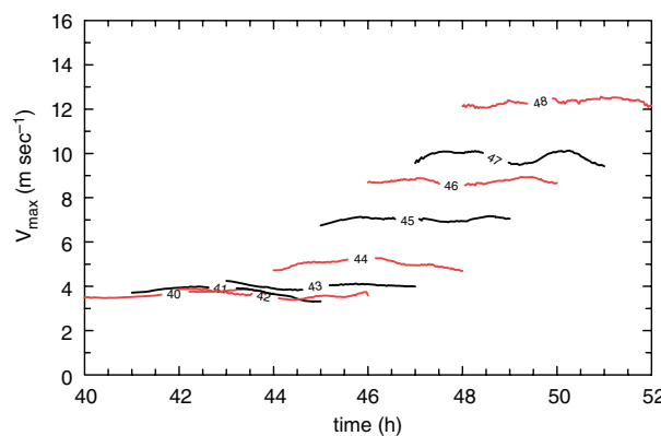
Figure 5. Time series of maximum azimuthally averaged tangential wind speed ( V_{\max} ) in the barotropic model within a radius of 40 km from the vortex centre. The curves are labelled with the barotropic model start time, initiated with the vorticity fields from the control simulation at these times. We focus on V_{\max} within a radius of 40 km to investigate any potential increases in V_{\max} due to barotropic processes near the circulation centre.
