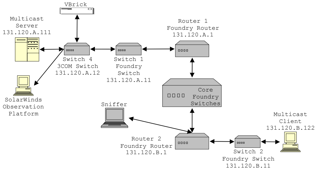
Figure 35. Network Diagram for the Stress Test
