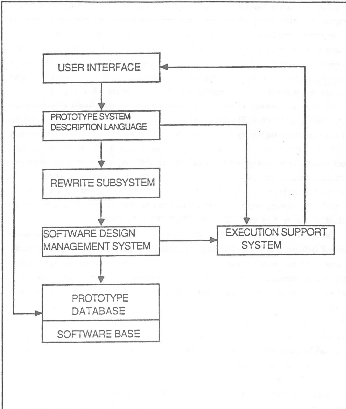
Figure 2. CAPS Architecture
