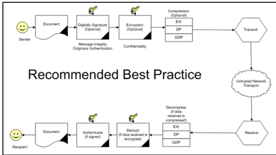
Figure 18. Composition of EXI Compression, XML Digital Signature, and XML Encryption as Recommended Best Practice for Secure and Efficient Messaging of Mission Orders to Unmanned Systems
