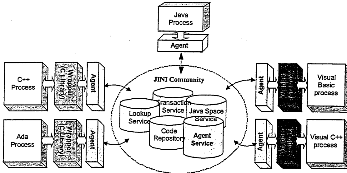
Figure 2. Agent wrappers
