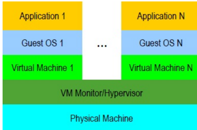
Figure 3. Server Virtualization [9]
