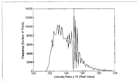
Figure 24. Rotor Pixel Frequency Versus Intensity Ratio ( I_r/I \times 70 )
