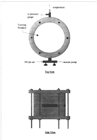
Figure 9. Calibration Chamber
