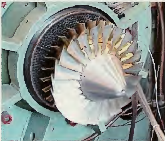
Figure 6. Rotor-Stator Assembly Prior to Casewall Installation
