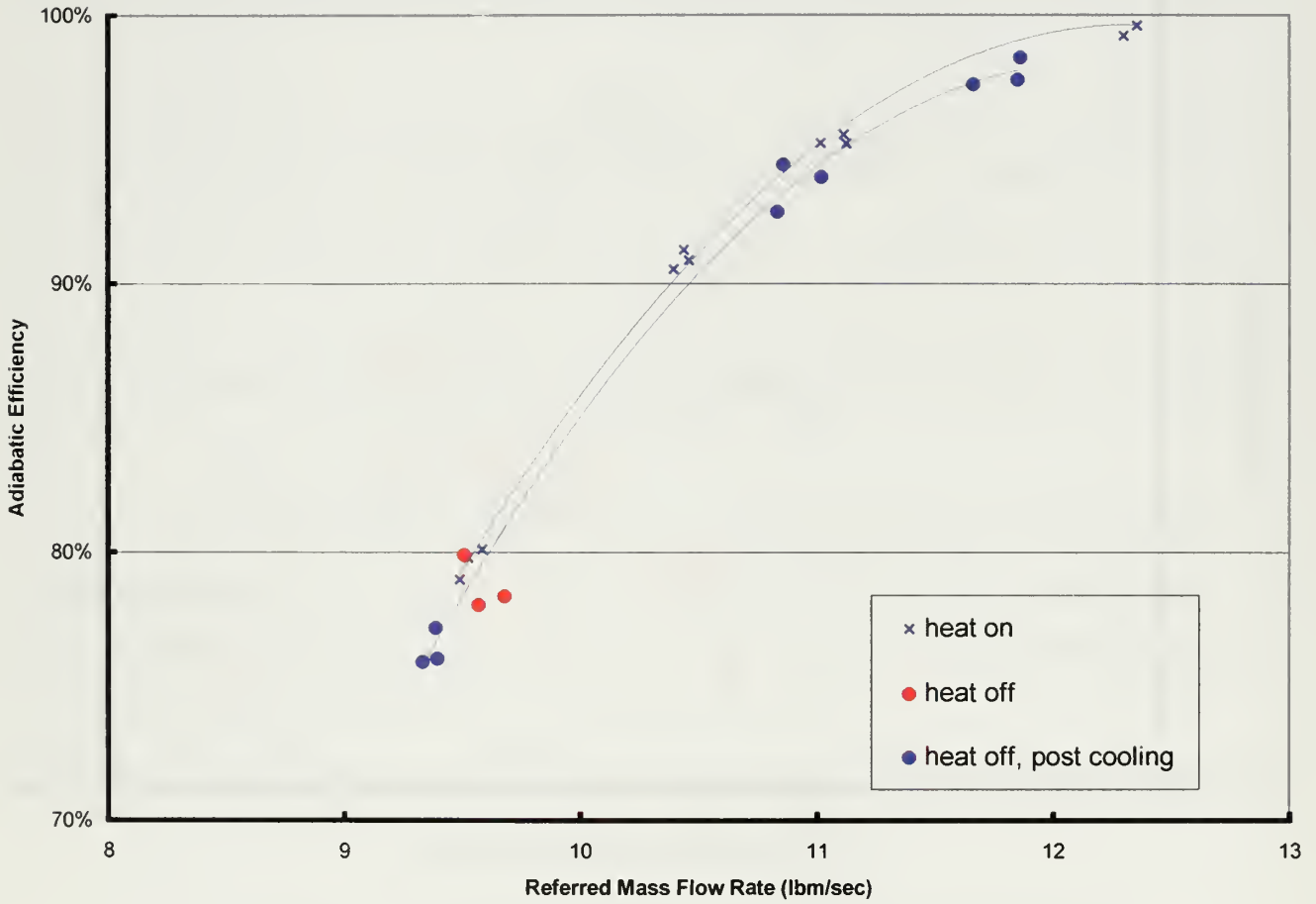
Figure 19. Adiabatic Efficiency ( \eta_1 ) vs. Referred Mass Flow Rate Effect of Casewall Temperature
