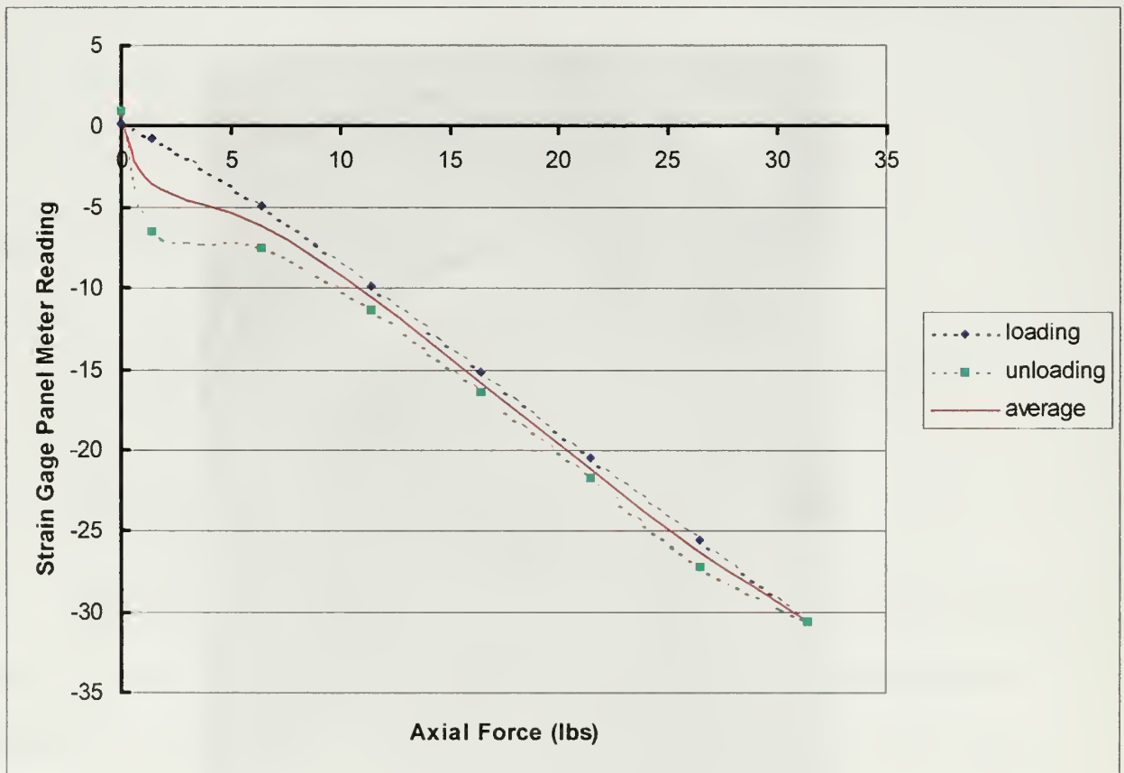
Figure B.4. Strain Gage Panel Meter Readings vs. Actual Axial Force
