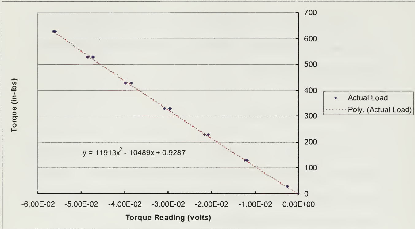
Figure B.2. Torque Calibration Data and Torque Coefficients
