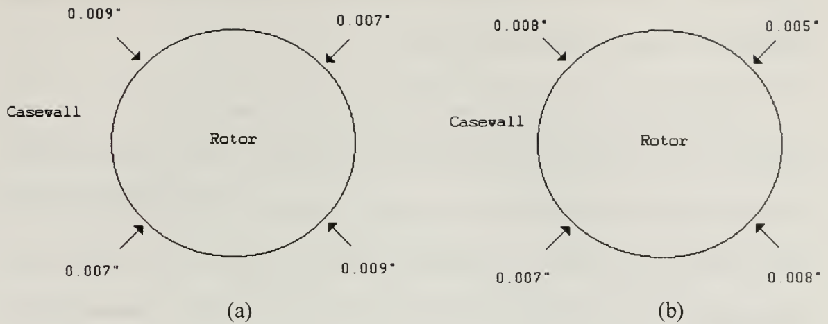
Figure 9. Tip Clearance between Rotor and Casewall Before (a) and After (b) Contact
