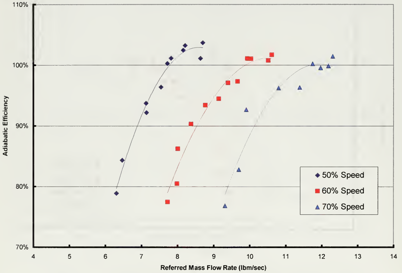
Figure 17. Adiabatic Efficiency ( \eta_2 ) vs. Referred Mass Flow Rate
