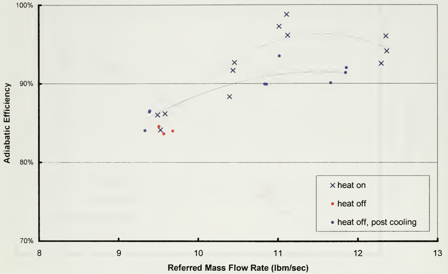
Figure 21. Adiabatic Efficiency ( \eta_3 ) vs. Referred Mass Flow Rate Effect of Casewall Temperature
