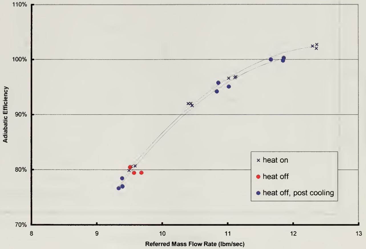
Figure 20. Adiabatic Efficiency ( \eta_2 ) vs. Referred Mass Flow Rate Effect of Casewall Temperature
