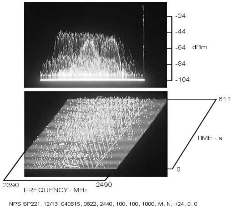
Figure 3 Occupancy and Use, Example 3
