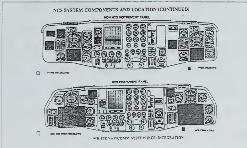
Figure 32 Cockpit Contrast
