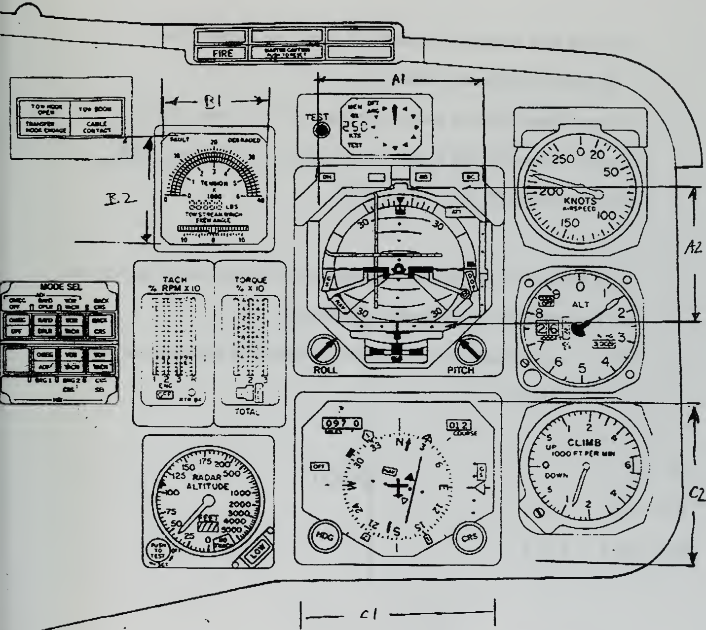
INSTRUMENT PANEL
