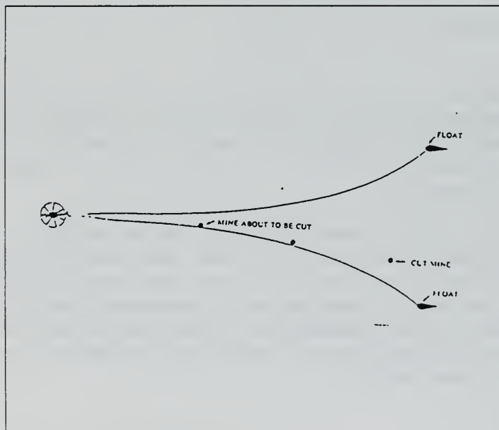
Figure 2 Mechanical Minesweeping
