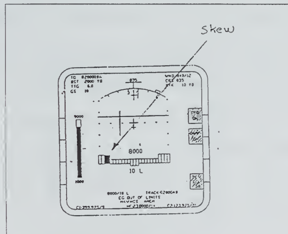
Figure 37 Skew Indication
