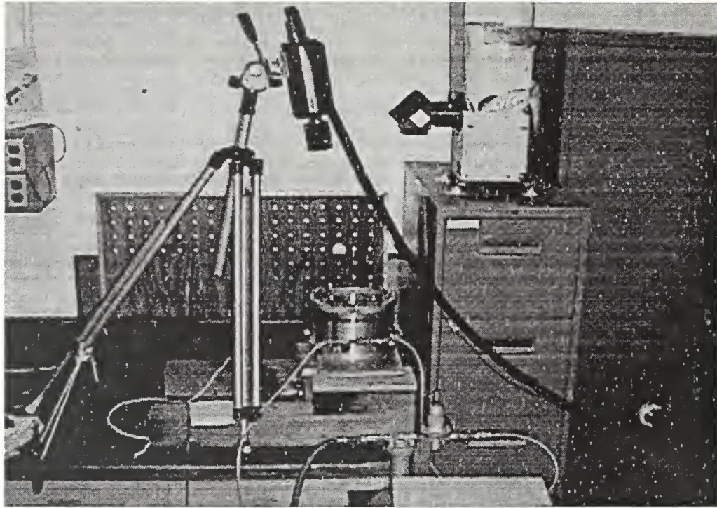
Figure 3. NPS PSP Calibration Experimental Setup
