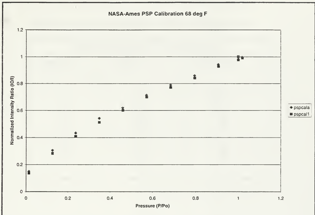
Figure D3. NASA-Ames PSP Calibration at 68° F
