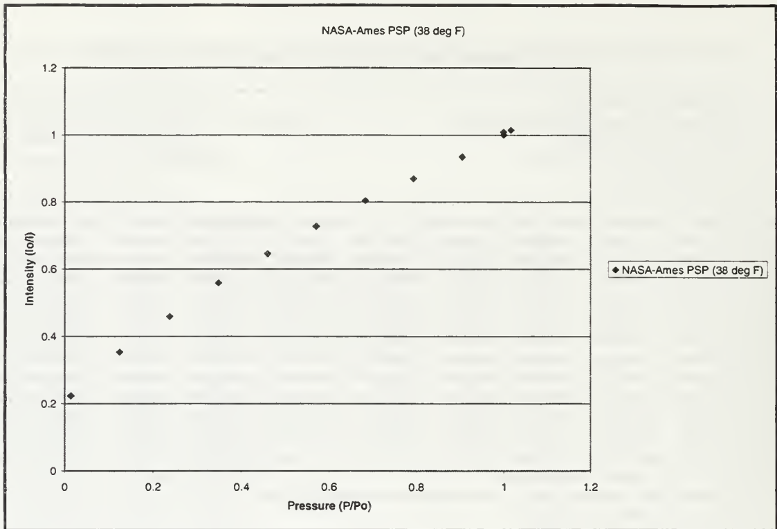
Figure D1. NASA-Ames PSP Calibration at 38° F
