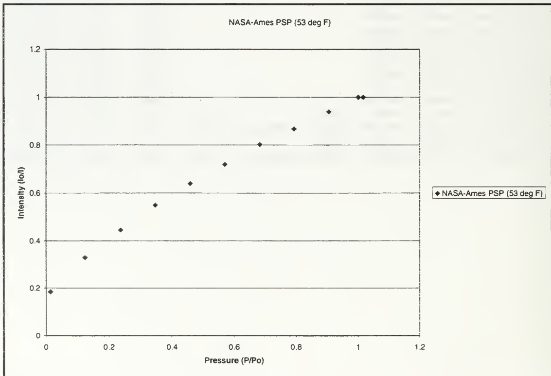
Figure D2. NASA-Ames PSP Calibration at 53° F
