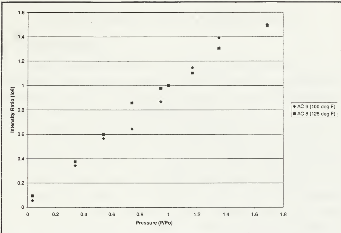
Figure 15. NPS Constant-Temperature, Variable-Pressure Repeatability (100°–125° F)
