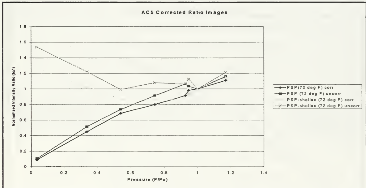
Figure C1. AC-5 Corrected Intensity Ratio
