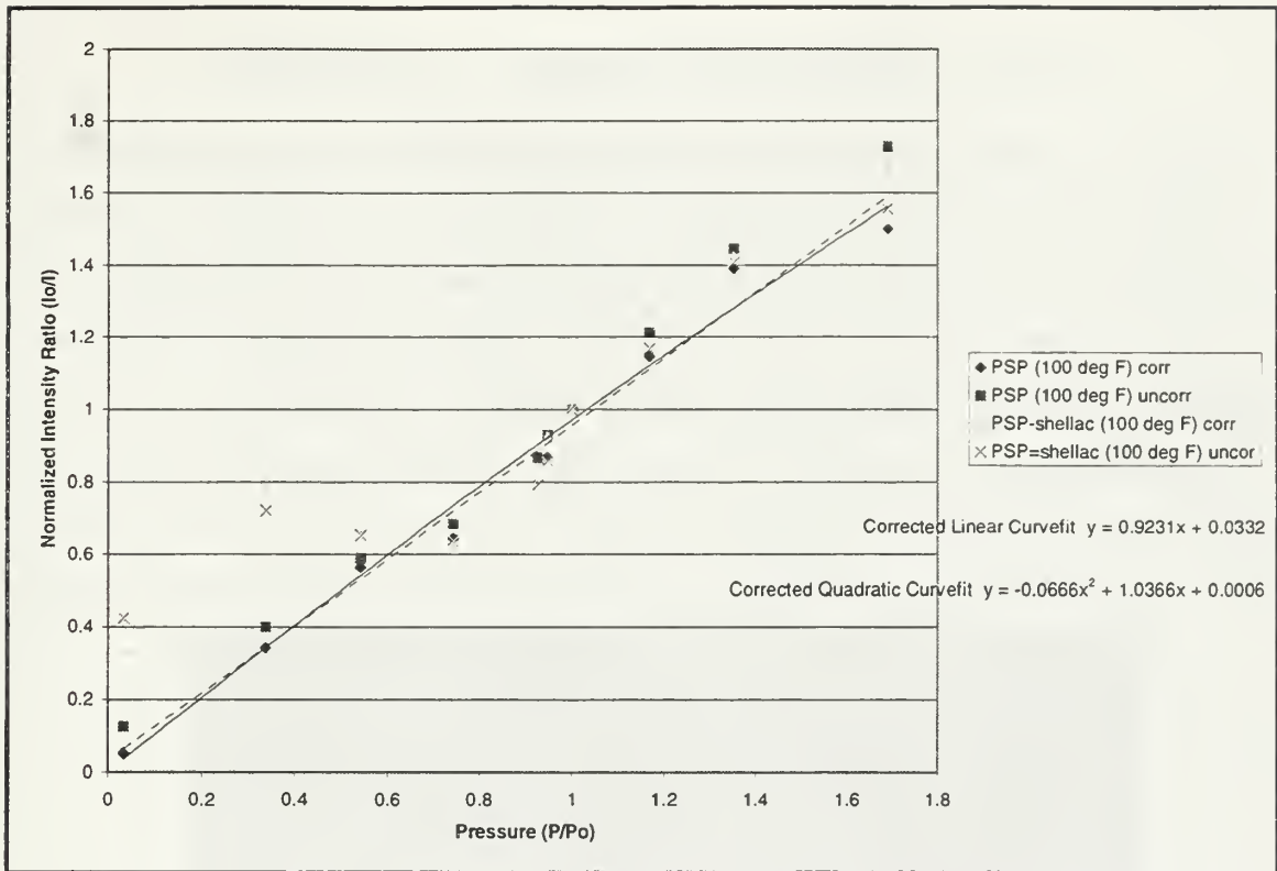
Figure F4. AC-9 Constant-Temperature, Variable-Pressure (100° F)
