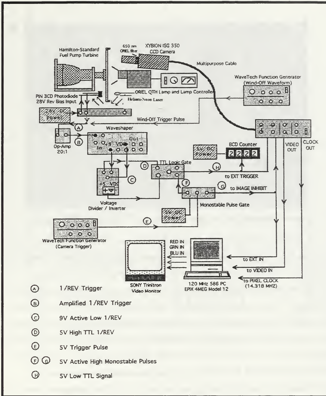
Figure 4. Image Acquisition System From Quinn [Ref. 3]
