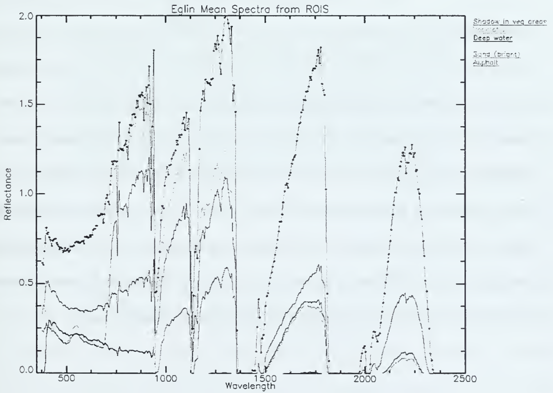
Figure 18. Mean Spectra for Regions of Interest
