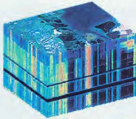
Figure 16. Sample Hyperspectral Data Cube (From Short, 1999)
