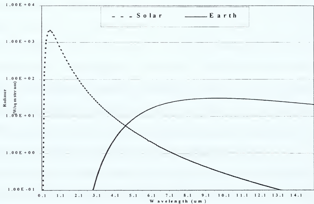
Figure 10. Planck’s Blackbody Radiation Curves for the Sun and the Earth Measured at the Earth’s Surface (After Gettys, 1989)
