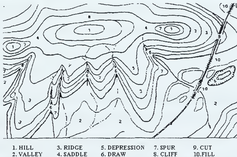
Figure 4. Terrain Feature Description Using Contour Lines (FM 21-26, 1993)
