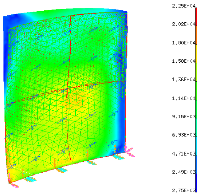
Figure 60. Structural Analysis, Optimized Blade
