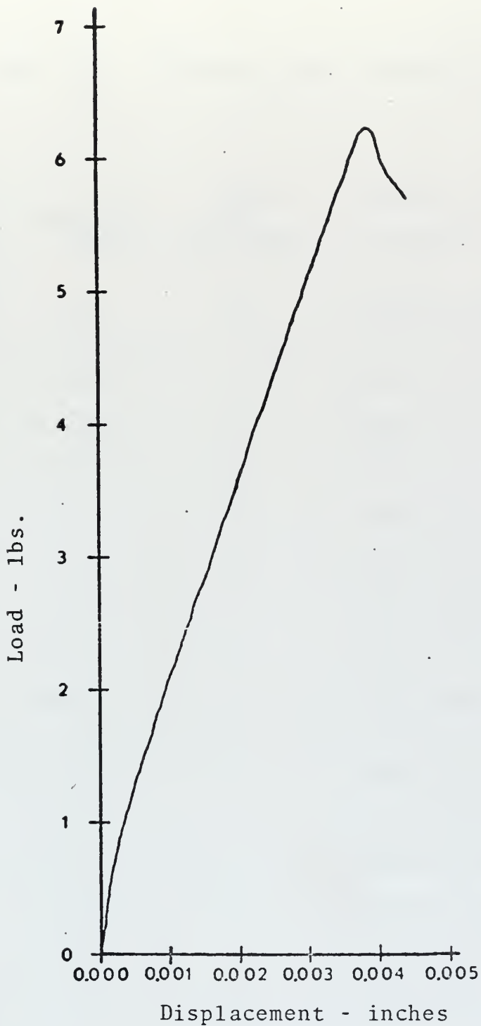
Figure 13. Load vs. Displacement plotted by an Instron testing machine using a strain gauge extensometer. Specimen was uncoated, treated in a \text{KNO}_3 bath at 365^\circ\text{C} . for sixty four hours, and had a crack length of 1.61 inches.
