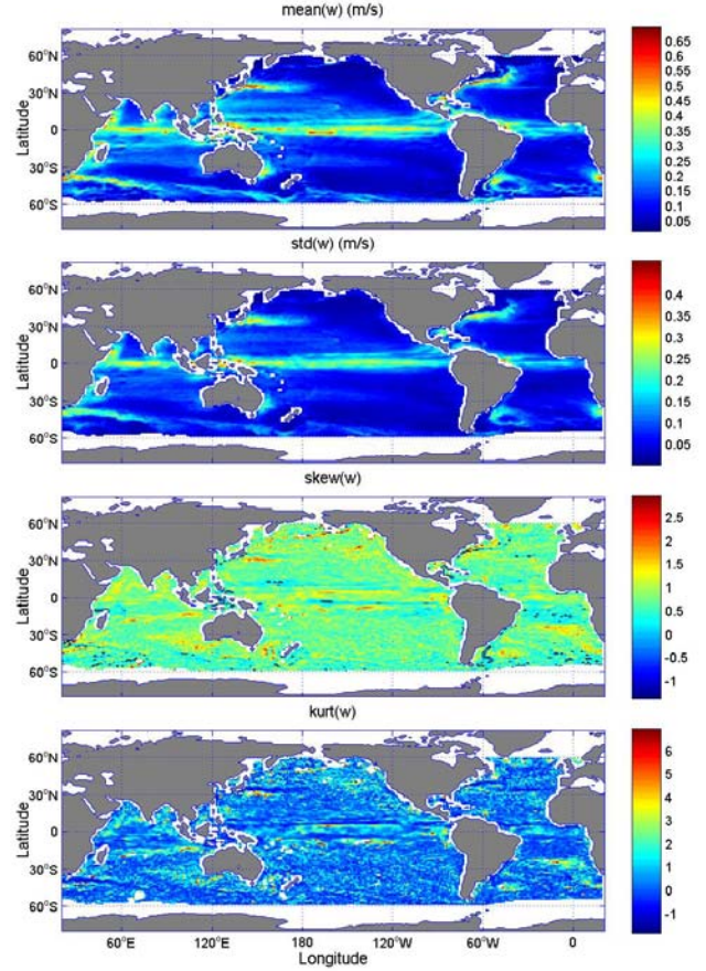
Figure 1. First four parameters of the surface current speeds calculated from the OSCAR data (1992-2007).
