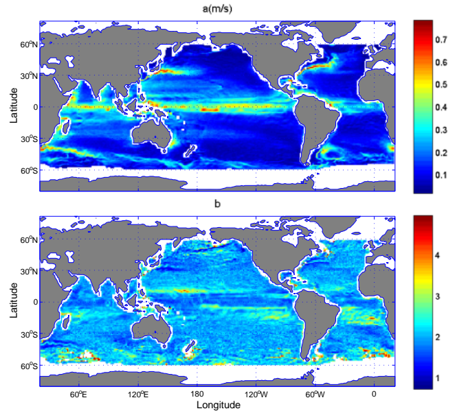
Figure 2. Same as in Fig. 1, but for Weibull parameters ( a , b ).
