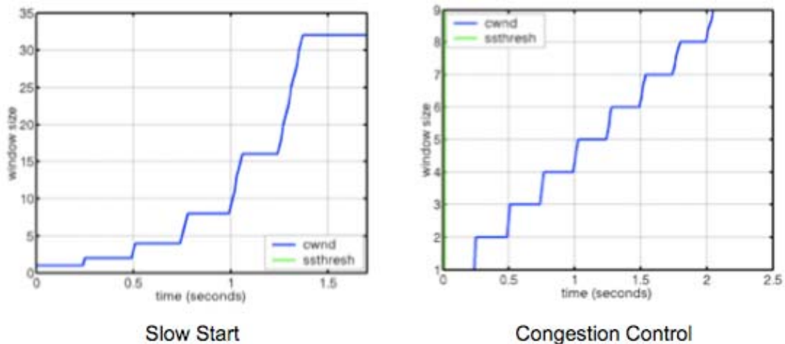
Figure 8. TCP Window Growth: Exponential vs. Linear (From Low, 2002, pp. 33, 35)
