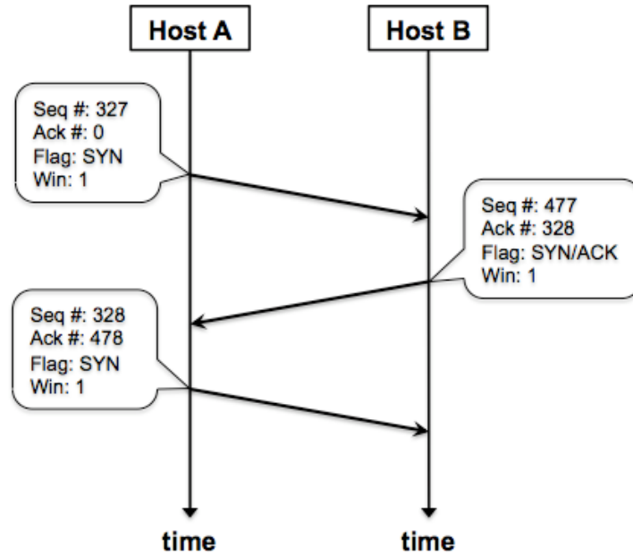
Figure 7. TCP 3-Way Handshake (From Fulp, 2009, p. 143)
