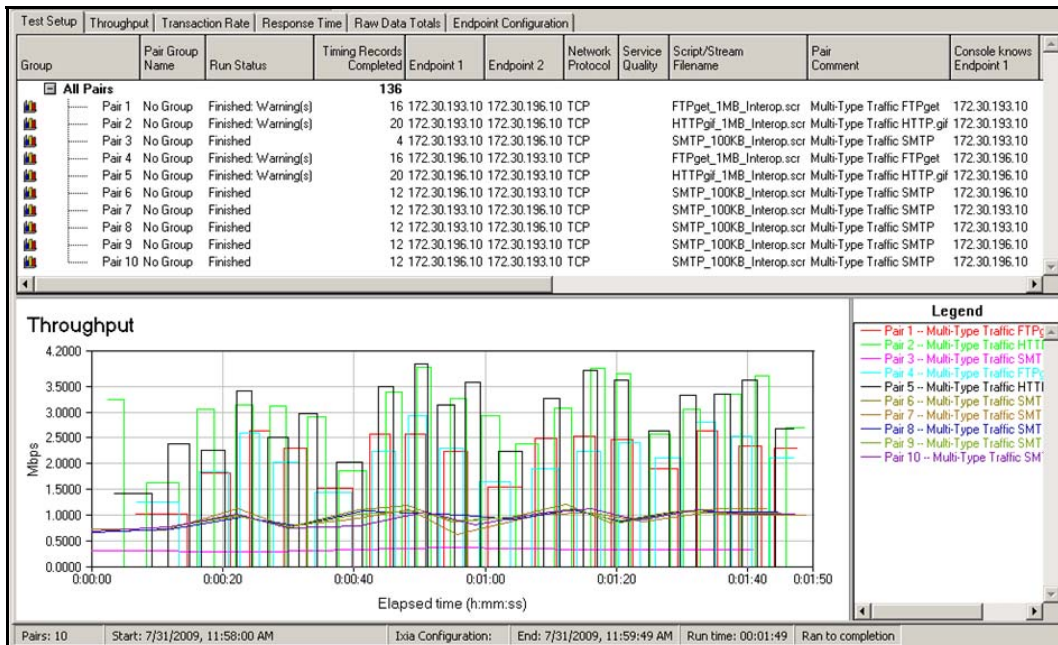
Figure 43. IxChariot GUI: Multi-User/Protocol/Direction, Cisco-WAAS
