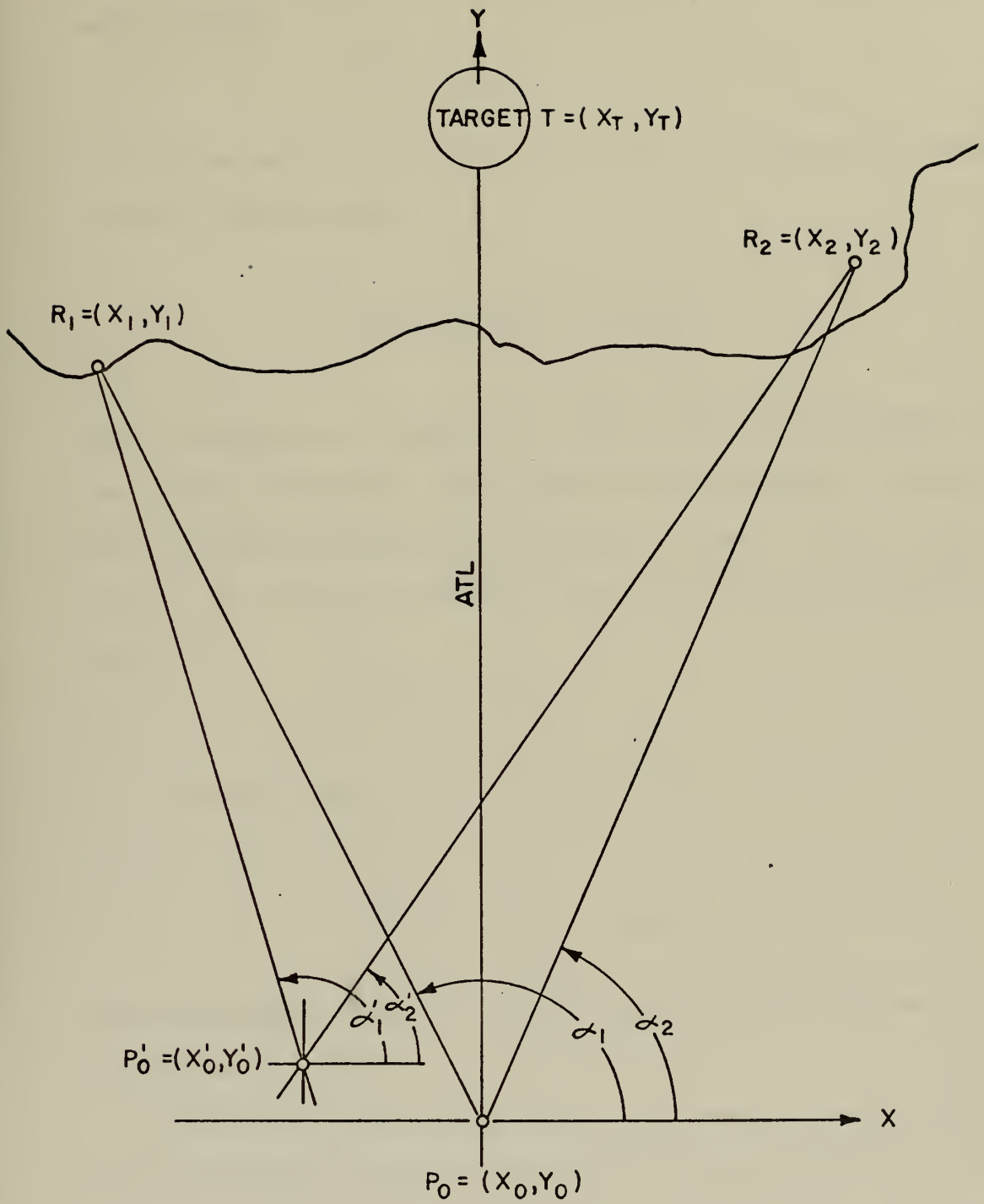
FIG.2 GEOMETRY FOR THE GYRO-PELORUS MODEL
