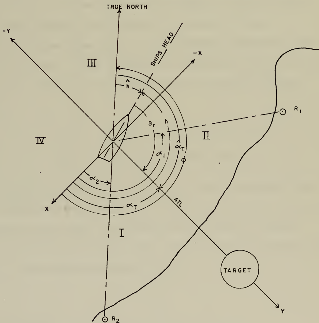
FIG. 1(c) RELATIONSHIP BETWEEN COORDINATE SYSTEMS
