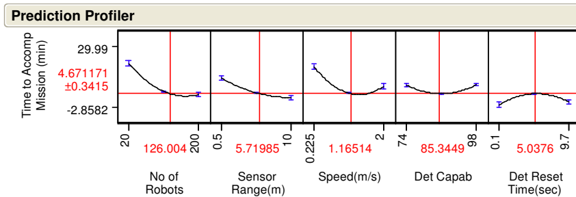
Figure 51. Prediction profiler from conditional regression of MOE 1 without noise factors
